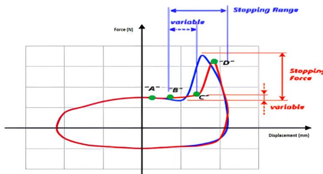
Figure 3. Hydraulic Rebound Stopper Diagram
